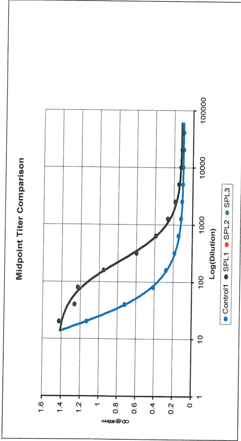
Curve Fit
